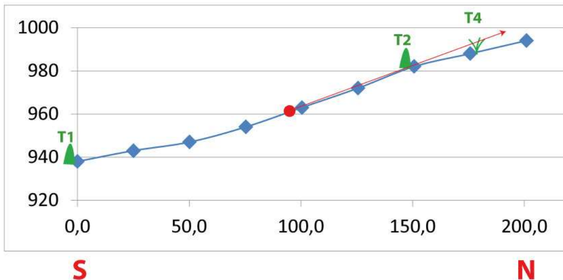
Figure 11 - Terrain profile of the line from South to North. Measured values from Google Earth.
